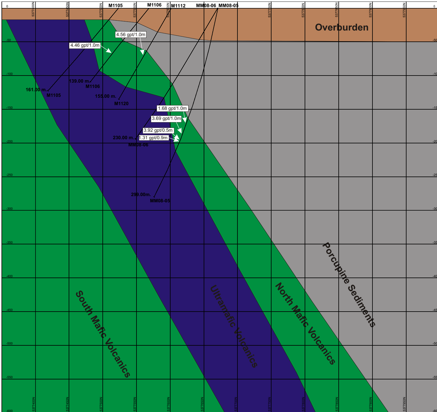
Schematic Section 494840E (Looking West)
