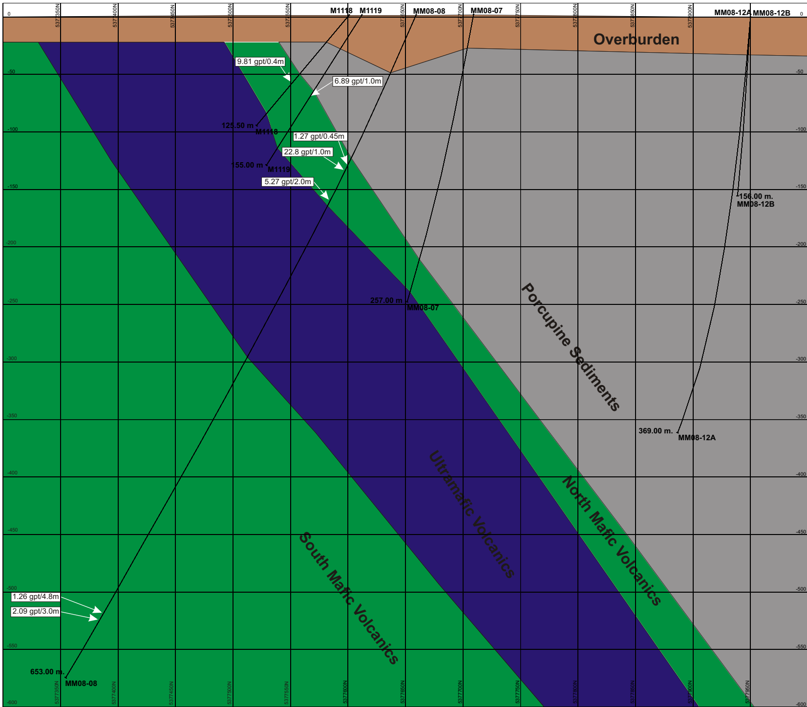
Schematic Section 494870E (Looking West)
